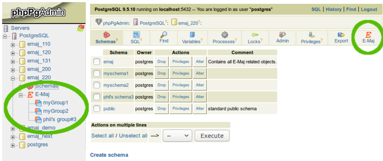
Fig. 32.1: Figure 1a – phpPgAdmin : connection to a database where E-Maj is installed.
