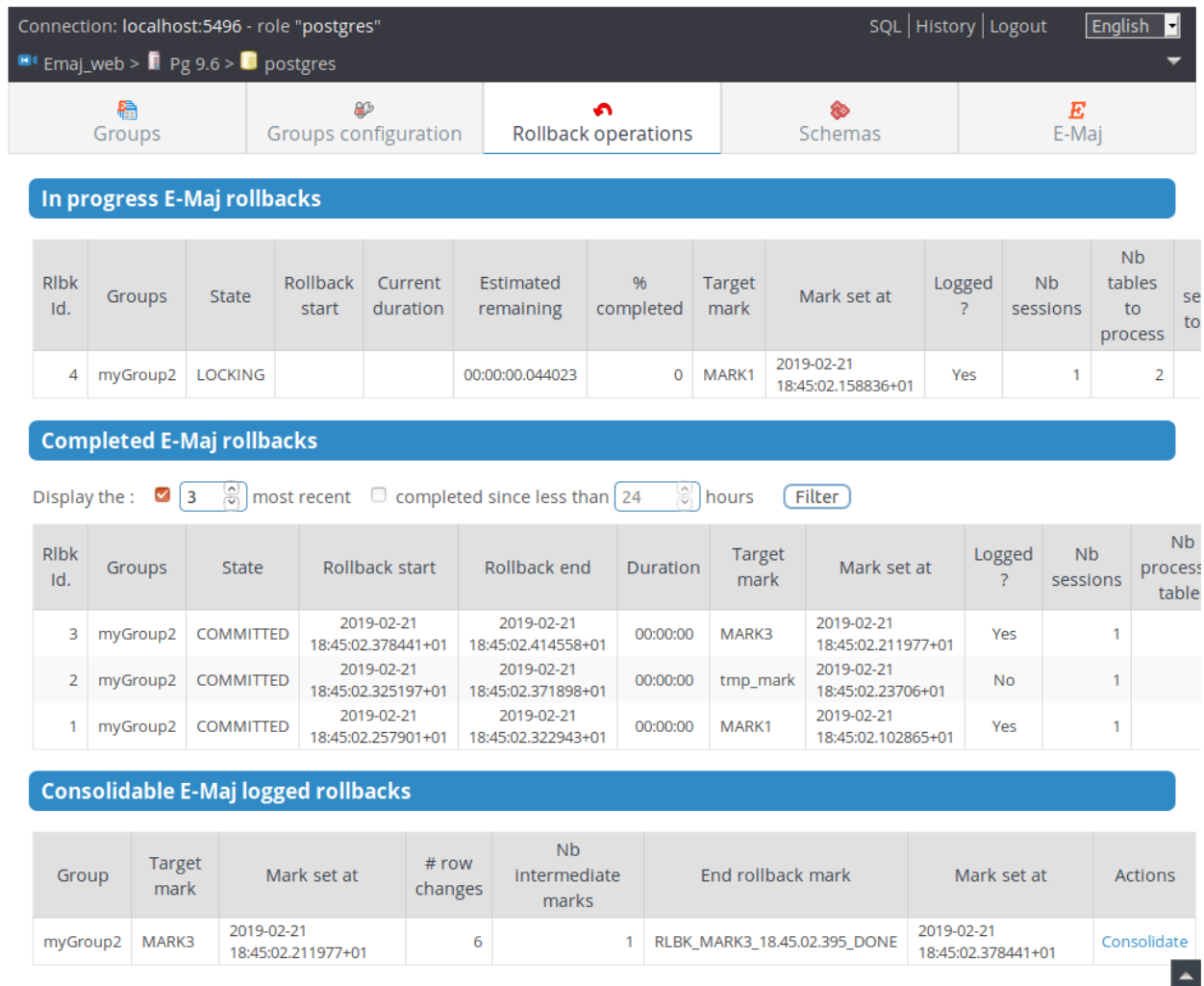
Fig. 11: Figure 11 – Rollback operations monitoring.
