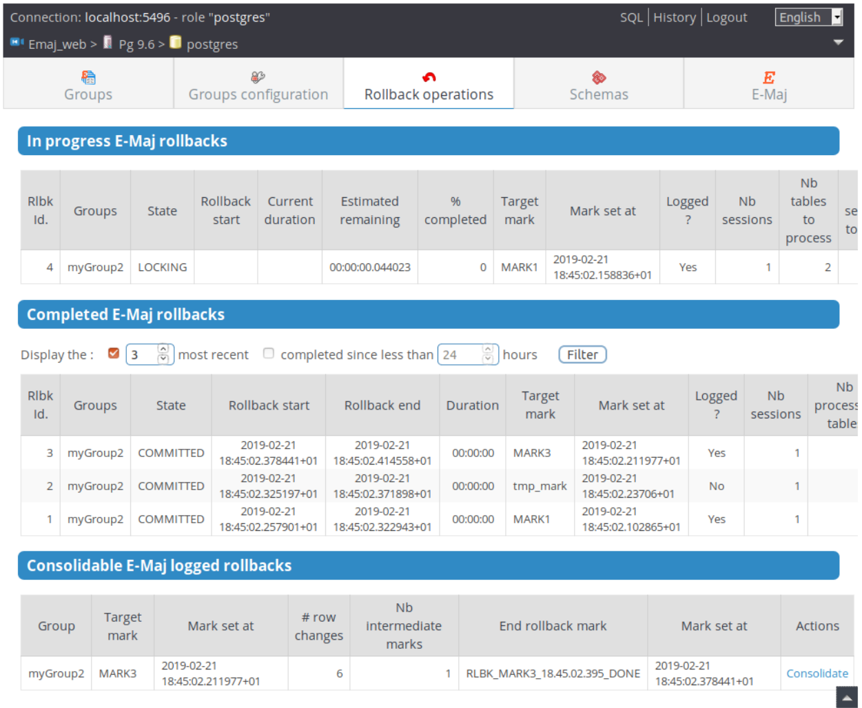
Fig. 12: Figure 12 – Rollback operations monitoring.
